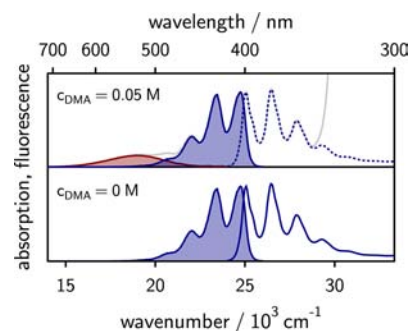
Figure 2. Absorption and emission spectra of 9,10-dimethylanthracene in the absence (bottom) and presence (top) of 0.05 M N,N -dimethylaniline. The solvent is a mixture of propyl acetate and butyronitrile of relative dielectric constant \epsilon_r = 14 (43 wt % butyronitrile). The emissions of the exciplex and the locally excited fluorophore are shaded in red and blue, respectively.
